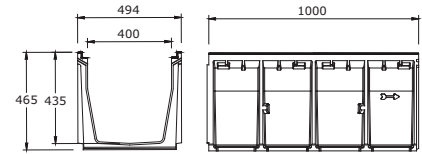
MEADRAIN ENS 4000
