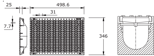
ENS 3000 ADA longitudinal cast iron grate 31/7,7 with PROFIX | PROFIX
