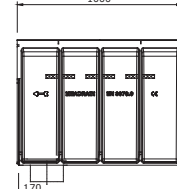
MEADRAIN EN 3000 with connection piece | MEADRAIN ENS 3070
