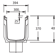
MEADRAIN EN 3000 with connection piece | MEADRAIN ENS 3070
